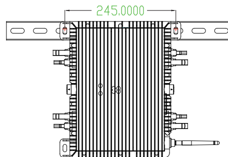
1300 / 1600 / 2000G3 (4MPPT) Mounting
